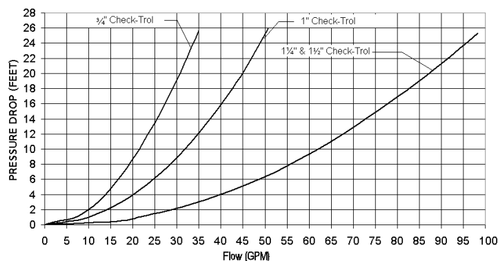
PERFORMANCE CURVE
